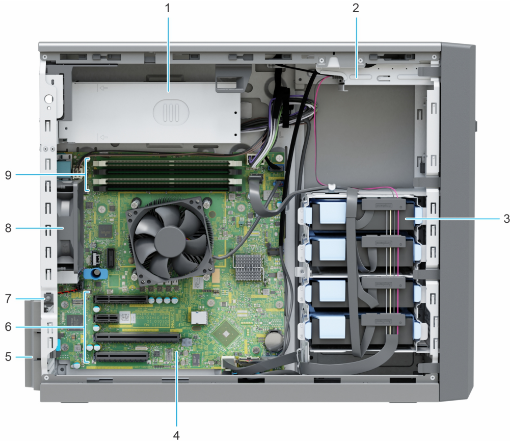
Figure 3. Inside view of the 4 x 3.5-inch drive system
